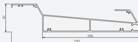
Chamber louvre
