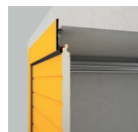
Installation in the opening – cover in front of the opening
