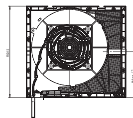
Straight box with an air inlet
