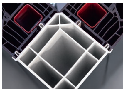
Coupling profiles
