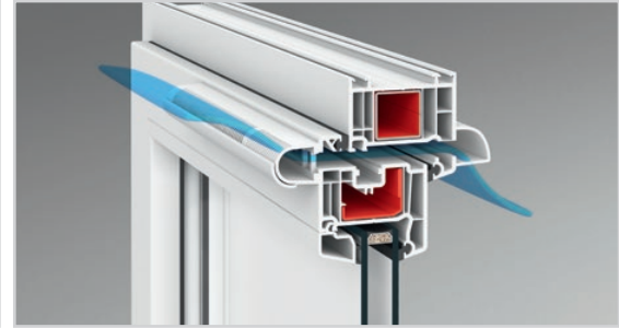
Aereco EMM pressure sensitive air inlet
