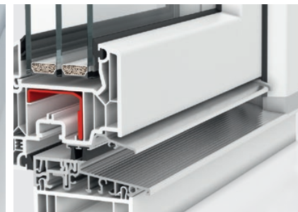
Low aluminium threshold
